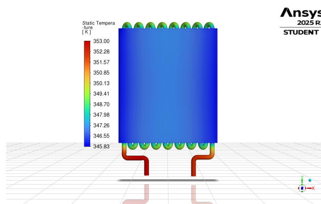
Fig. 11. Ethylene-glycol velocity inlet 1,5 m/s
