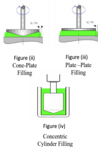
Fig. 2. Experimental setup (i) modular compact rheometer (ii) Cone Plate Filling (iii) Plate-Plate filling (iv) Concentric Cylinder Filling
