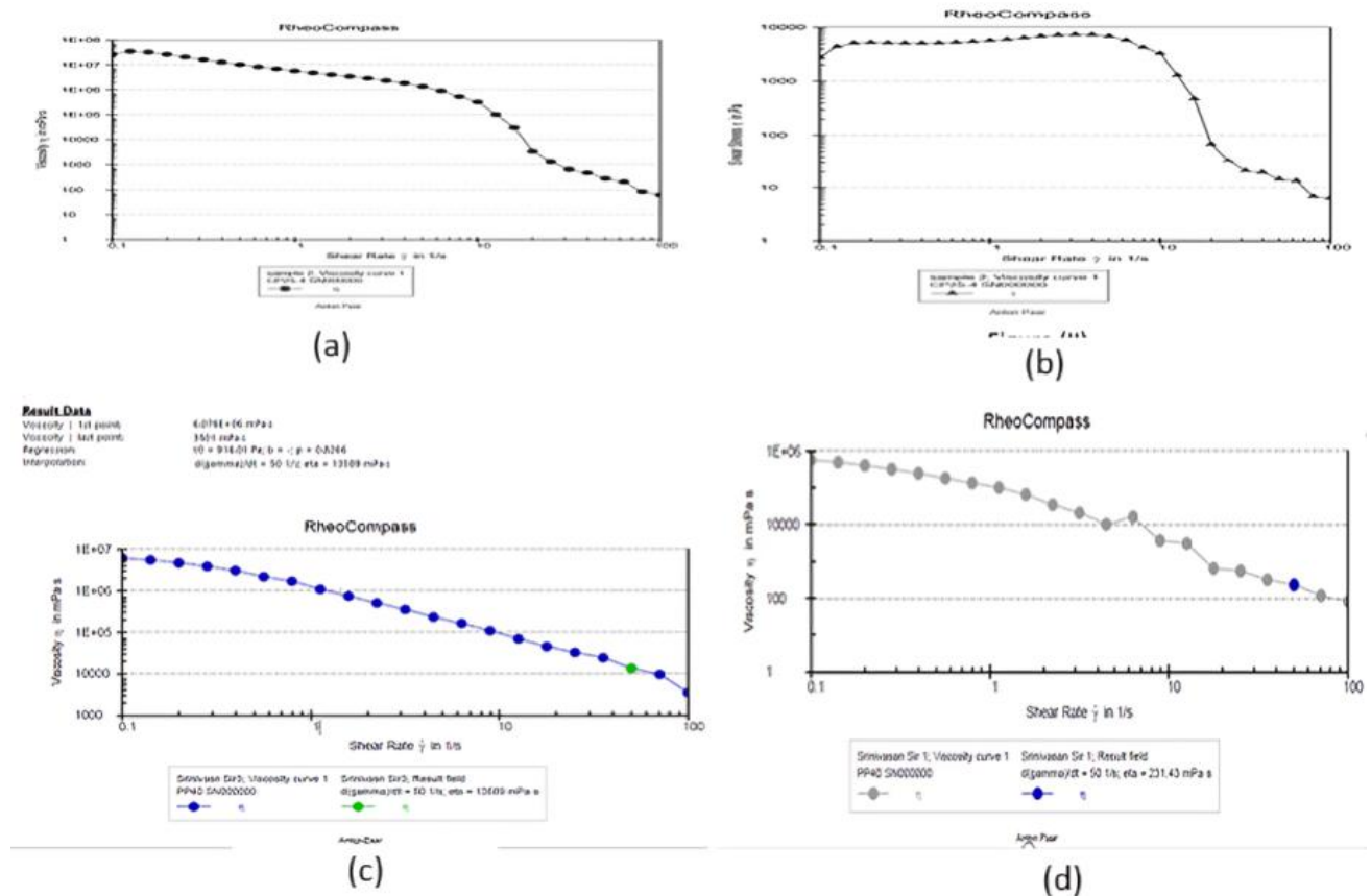
Fig. 6 Viscosity vs strain rate for 30 days old sample for VMAF Media, Gel and polymer 6 (i) Viscosity vs strain rate for 30days old VMAF sample (ii) Shear stress vs strain rate for a 30-day old sample of VMAF (iii) Viscosity vs Strain rate for gel (iv) Viscosity vs strain rate for polymers
